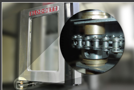
Triple mount door with turnbuckle
